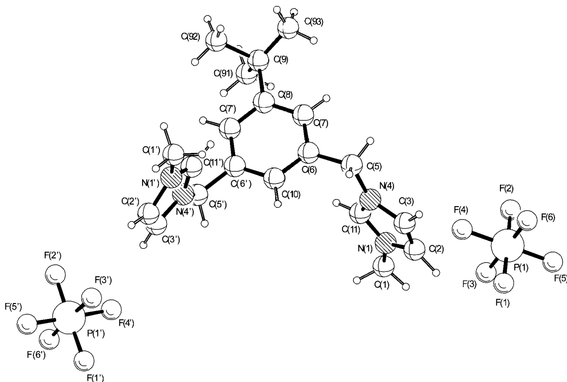
Figure 2. Molecular structure of 1b ·2PF 6
