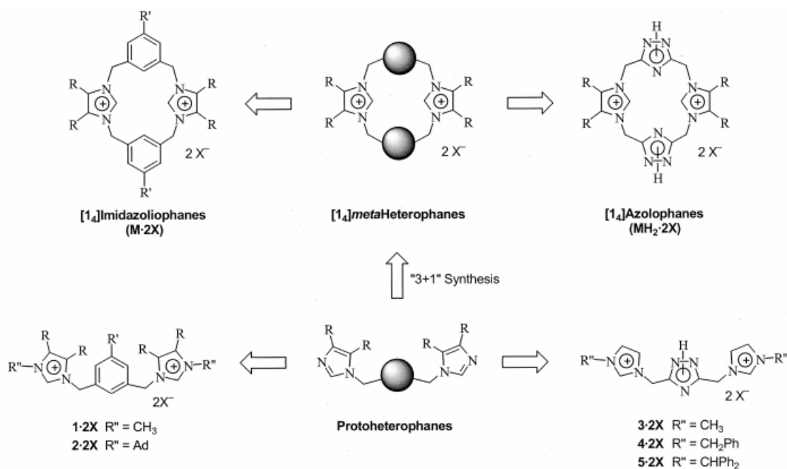
Figure 1 From protoheterophanes to dicationic protoheterophanes and their incorporation into [1 4 ]metaheterophanes
