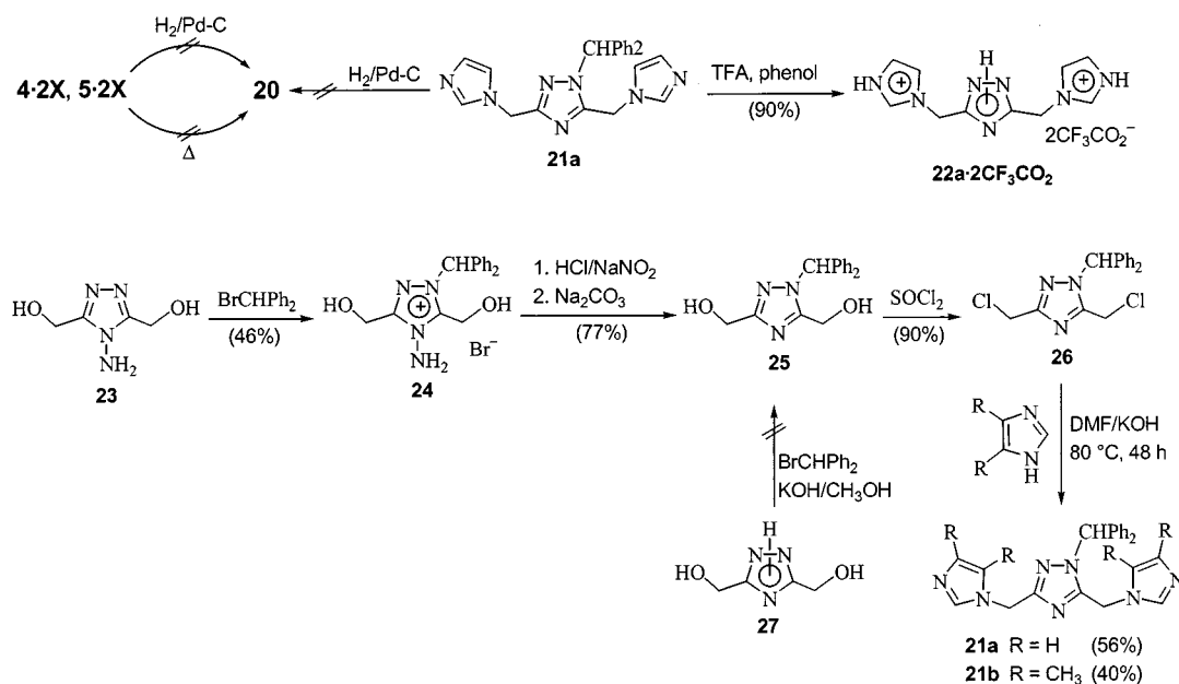
Scheme 4. Synthesis and dequaternization of N -benzhydrylprotophanes 21
