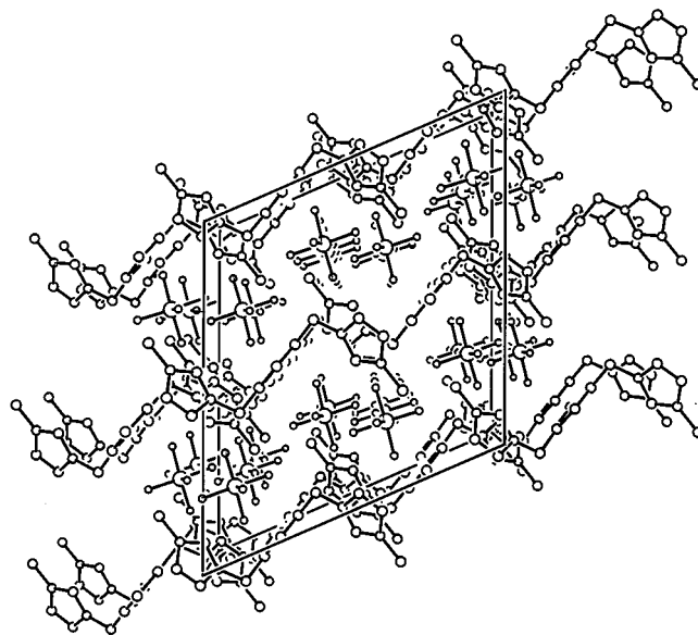
Figure 3. Packing of dicationic protophane 1b ·2PF 6 viewed along the crystallographic b axis
