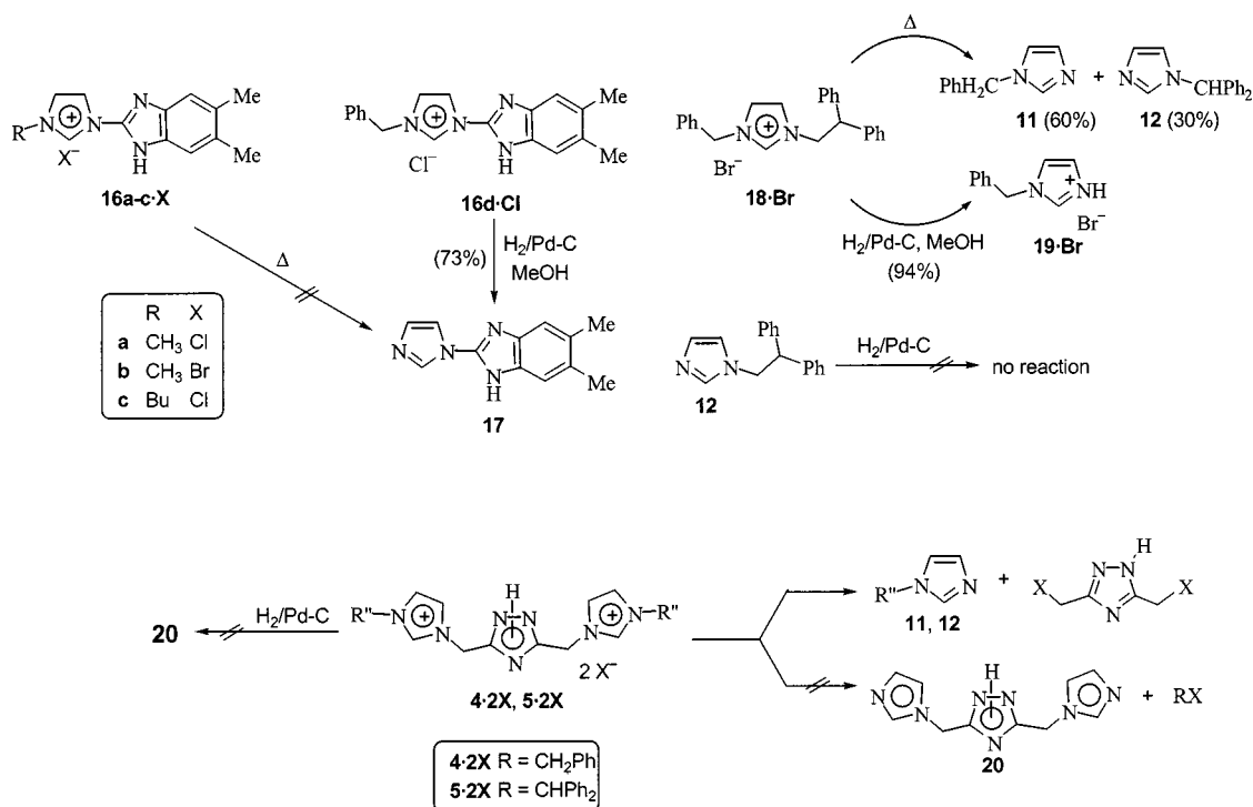
Scheme 3. Dequaternization reactions of azolium salts 16·X , 18·Br and dicationic protophanes 4·2X , 5·2X
