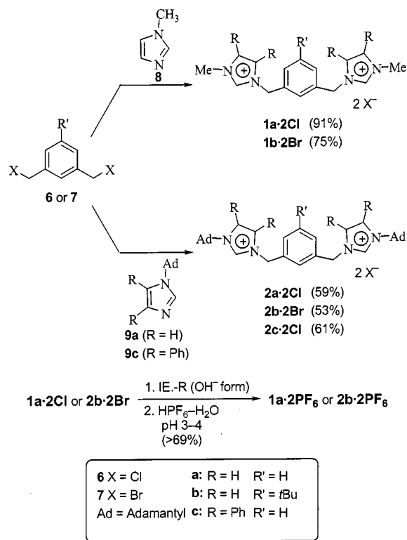
Scheme 1. Synthesis of dicationic protophanes 1·2X and 2·2X
