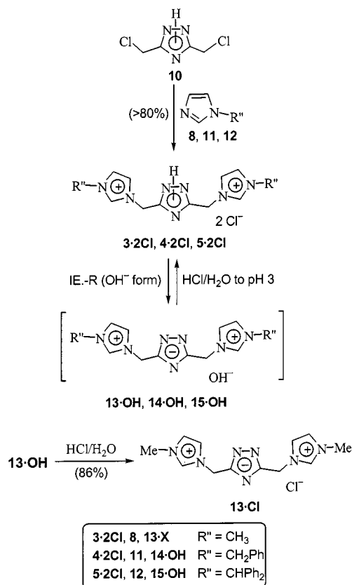
Scheme 2. Synthesis of proton-ionizable dicationic protophanes 3·2X–5·2X and their corresponding betaines 13·X–15·X
